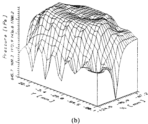
Fig. 12 Contact pressure developed on a pad at (a) 30 seconds, and (b) 120 seconds
