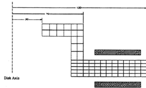
Fig. 10 A disk model used for analyzing heat transfer in a disk brake assembly with FFT-FEM program
