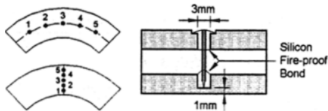
Fig. 2 Thermocouple locations and installation in the brake disc and pads
