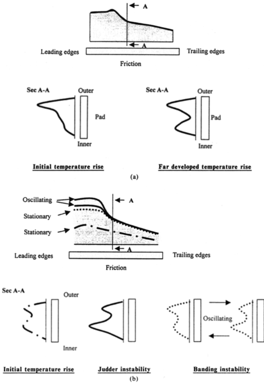
Fig. 7 Schematics of temperature profiles measured on friction pad: (a) stable distribution and (b) unstable distribution
