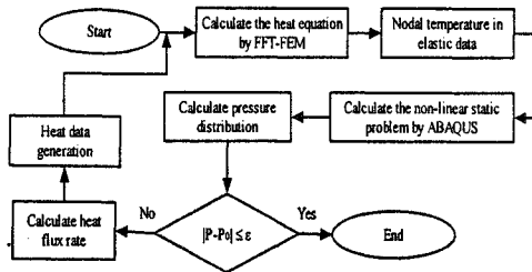
Fig. 3 Thermo-elastic simulation algorithm by using combined FFT-FEM(for heat transfer) and ABAQUS TM (for elastic analysis)
